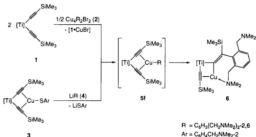
Scheme 1. Synthesis of the 1,1-bis-metalla alkenyl complex 6 ; (\eta^5-C_5H_4SiMe_3)_2Ti is abbreviated as [Ti].
